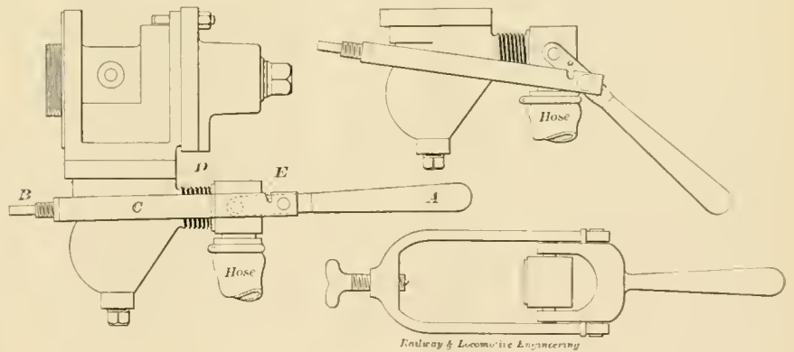
TRIPLE VALVE TESTING APPLIANCE.
